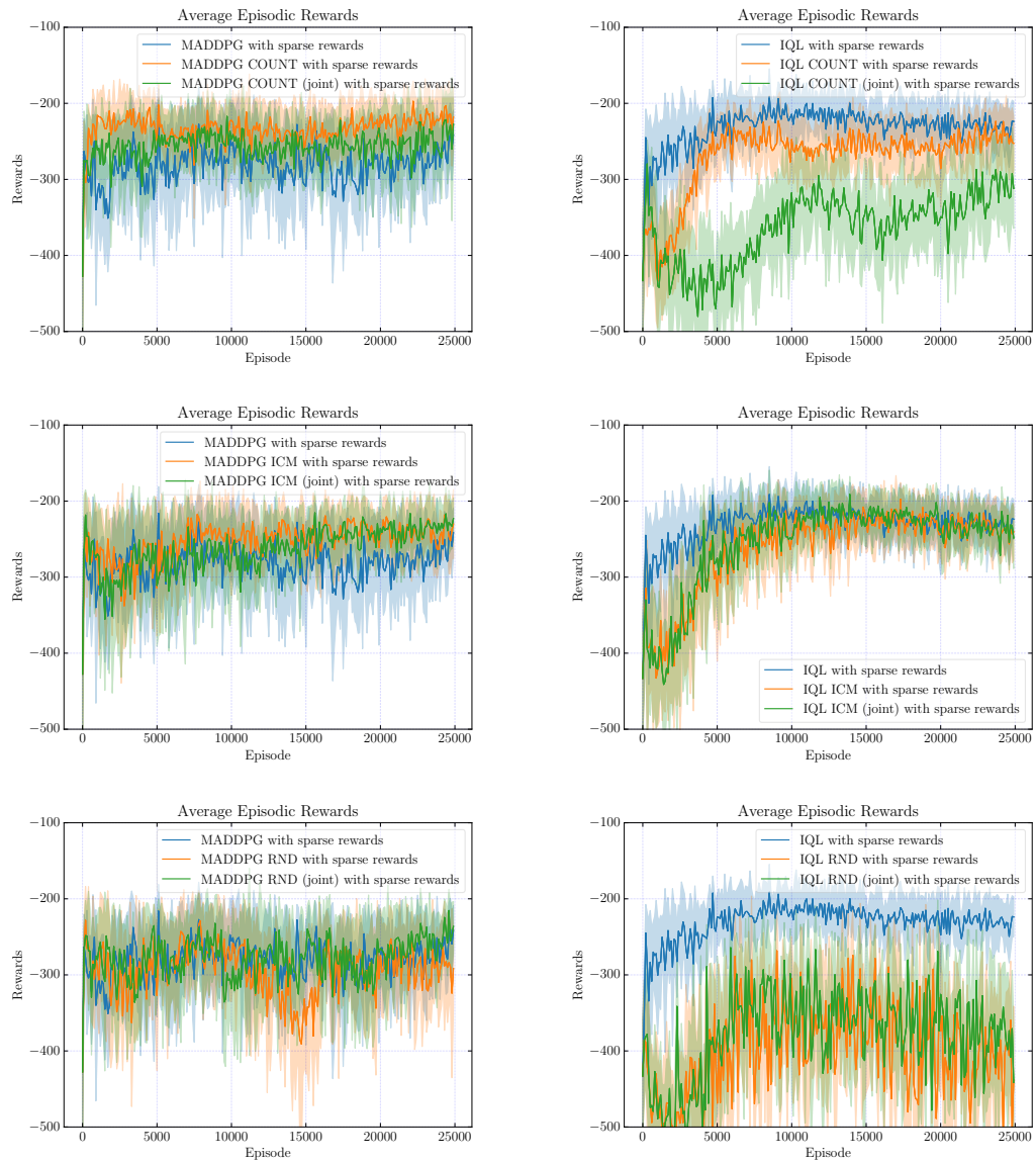
Figure C.15: Episodic rewards for MADDPG (left column) and IQL (right column) with individual and joint curiosities for cooperative navigation task with sparse rewards.
