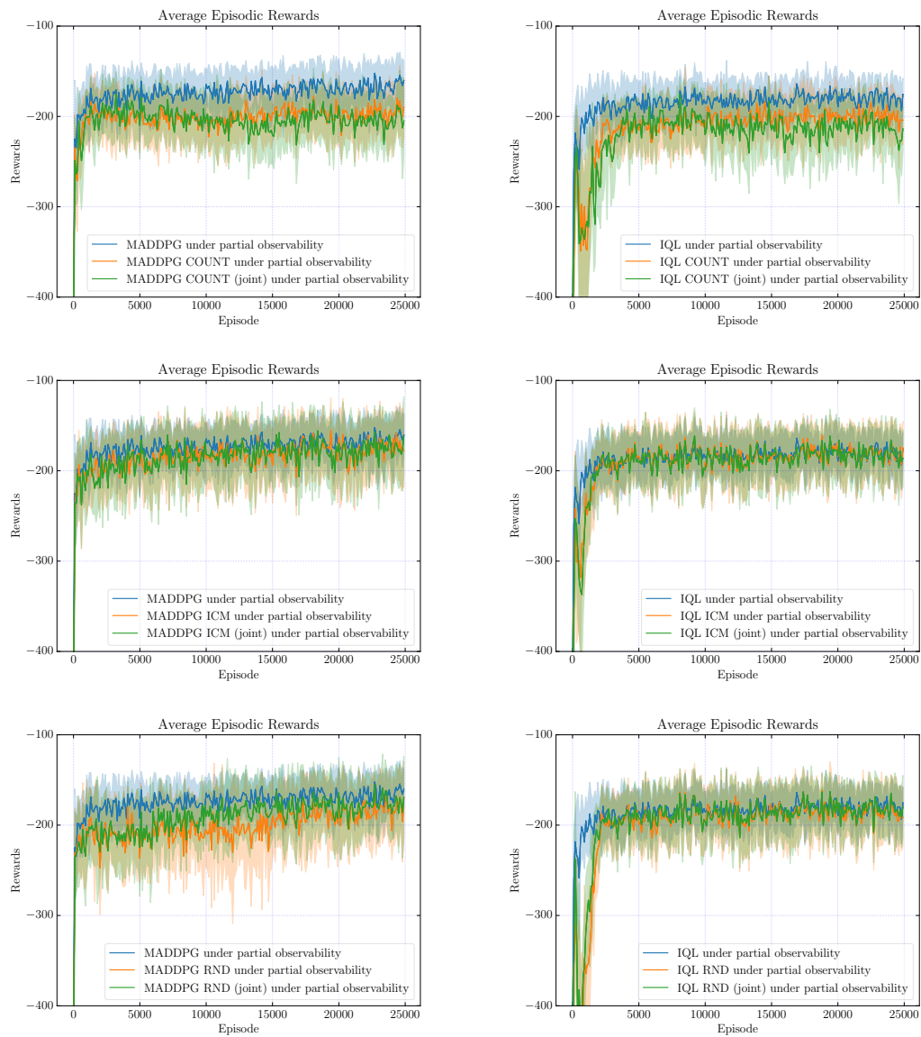
Figure C.7: Episodic rewards for MDDPG (left column) and IQL (right column) with individual and joint curiosities for cooperative navigation task under partial observability.
