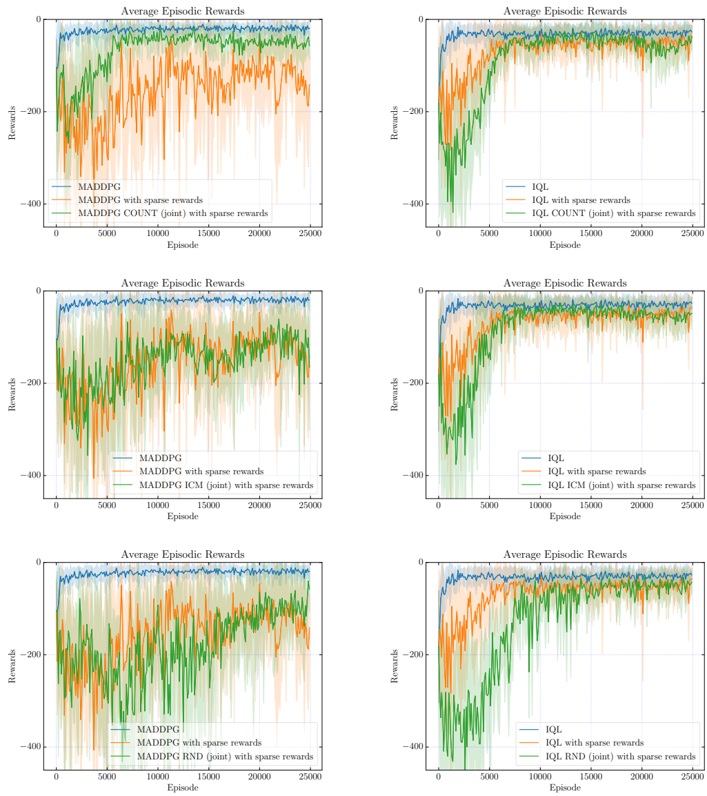
Figure C.14: Episodic rewards for MADDPG (left column) and IQL (right column) with joint curiosities for cooperative communication task with and without sparse rewards.
