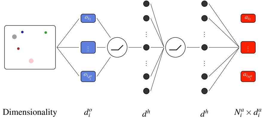
Figure 3.3: Illustration of MADDPG actor architecture for agent i with two intermediate layers of hidden representation size d^h and ReLU activation function.
