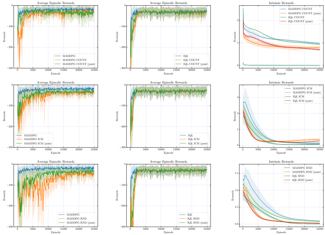
Figure 4.5: Episodic reward of MADDPG (left column) and IQL (middle column) with individual and joint count (1st row), ICM (2nd row) and RND (3rd row) curiosity on the cooperative communication task. The right column shows intrinsic rewards for MADDPG and IQL with the respective curiosity applied individually and jointly.
