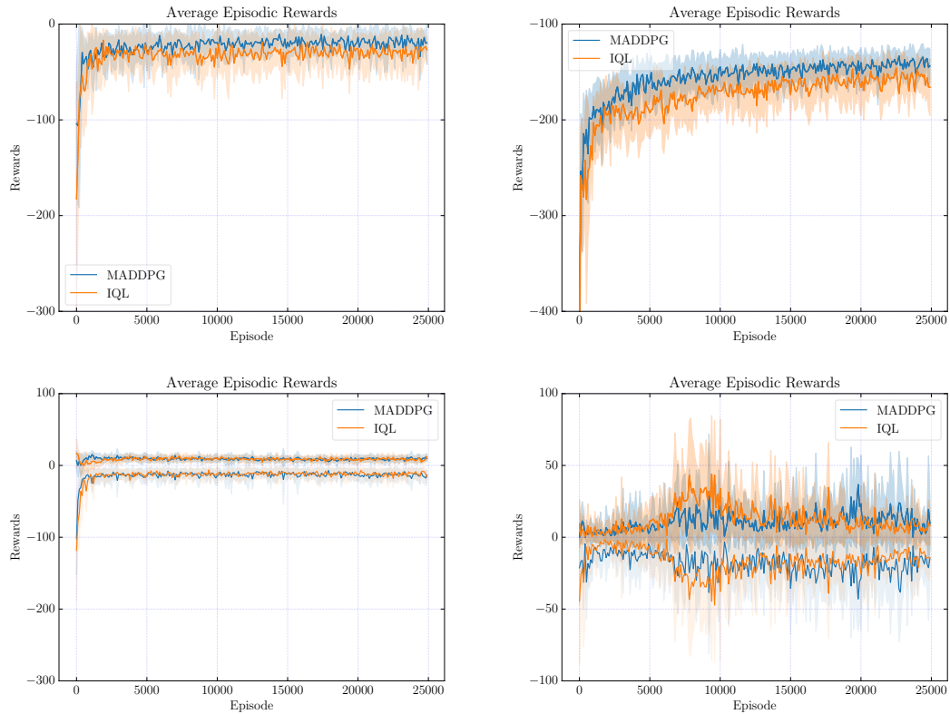
Figure 4.4: Episodic reward of baselines MADDPG (blue) and IQL (orange) for cooperative communication (top left), cooperative navigation (top right), physical deception (bottom left) and predator-prey task.
