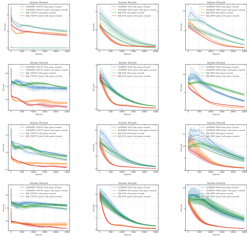
Figure C.23: Intrinsic rewards for MADDPG and IQL with individual and joint curiosities for cooperative communication (1st row), cooperative navigation (2nd row), physical deception (3rd row) and predator prey (4th row) task with sparse rewards.
