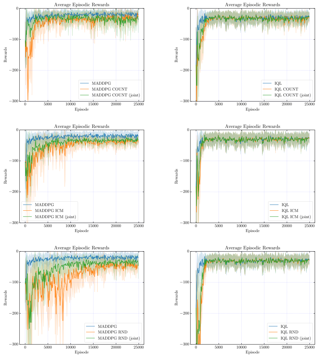
Figure C.1: Episodic rewards for MDDPG (left column) and IQL (right column) with individual and joint curiosities for cooperative communication task.
