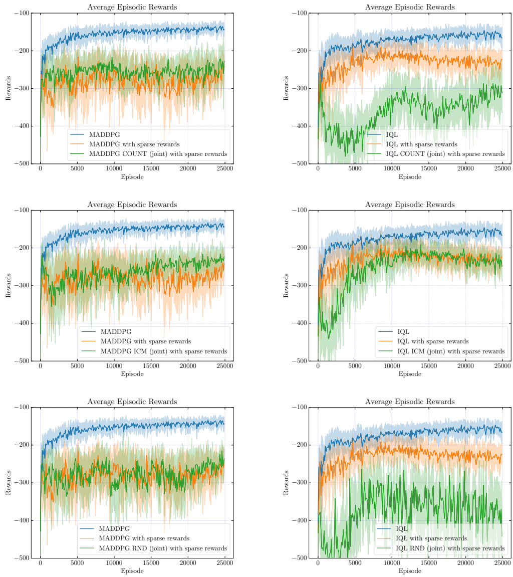
Figure C.16: Episodic rewards for MADDPG (left column) and IQL (right column) with joint curiosities for cooperative navigation task with and without sparse rewards.
