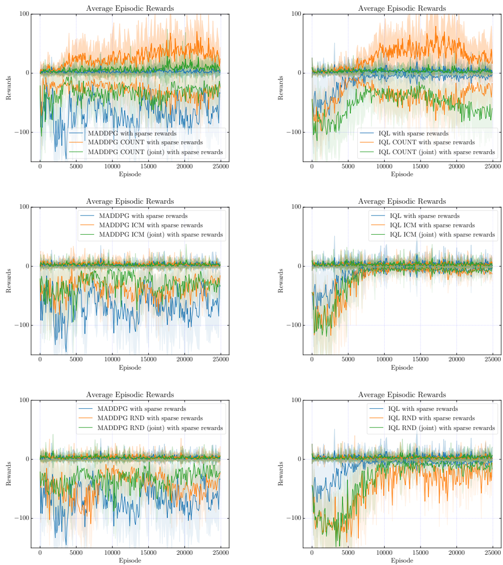
Figure C.19: Episodic rewards for MADDPG (left column) and IQL (right column) with individual and joint curiosities for predator prey task with sparse rewards.
