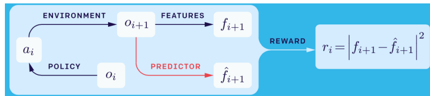
Figure 2.5: Outline of the feature prediction computed by RND. The trained predictor network computes its predicted representation solely relying on observation o_{i+1} . Figure taken from OpenAI [2018b]
