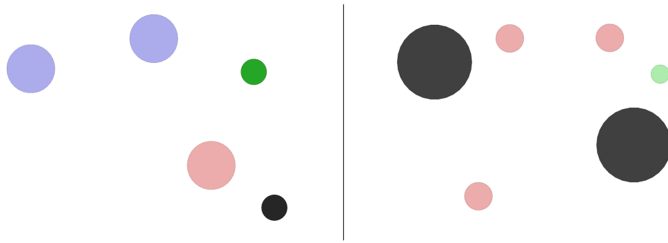
Figure 4.2: Rendering of physical deception (Left) and predator-prey (Right) environments. (Left) The collaborating agents (blue) have to move to the goal landmark (green) while deceiving the adversary agent (red). (Right) The adversary agents (red) aim to catch the faster fleeing agent (green).
