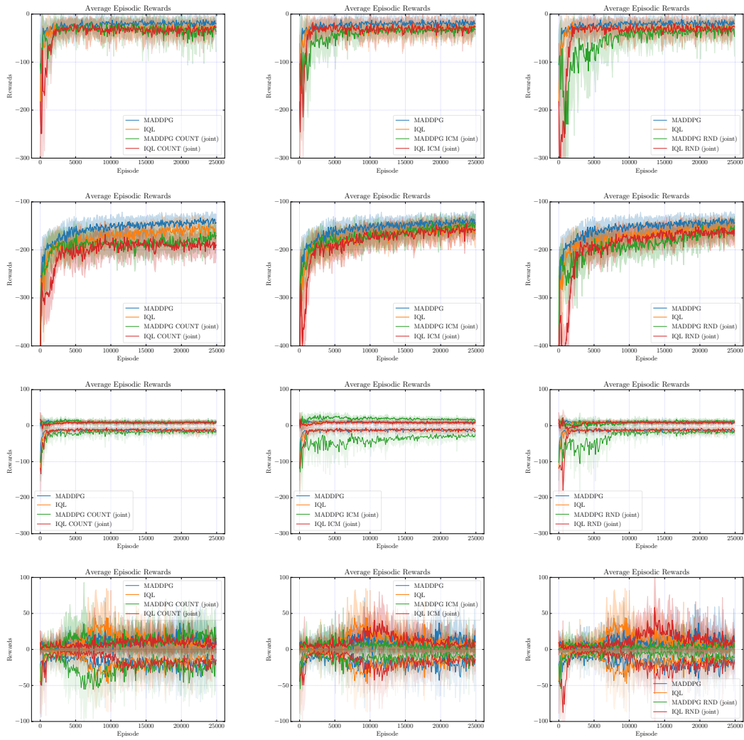
Figure 4.6: Episodic reward of baselines MADDPG and IQL compared with count, ICM and RND curiosity for cooperative communication (1st row), cooperative navigation (2nd row), physical deception (3rd row) and predator-prey (4th row) task.
