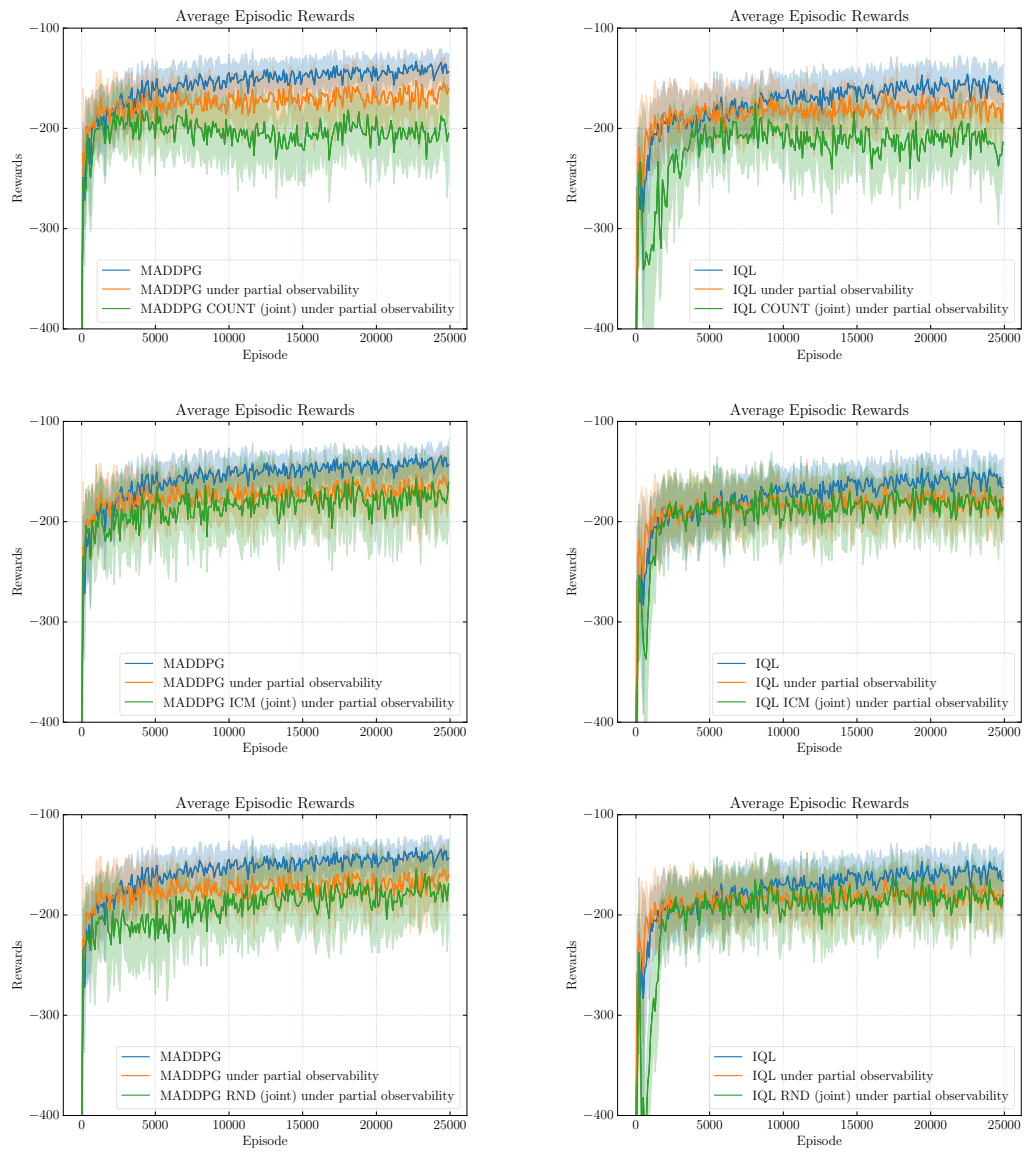
Figure C.8: Episodic rewards for MADDPG (left column) and IQL (right column) with joint curiosities for cooperative navigation task with and without partial observability.
