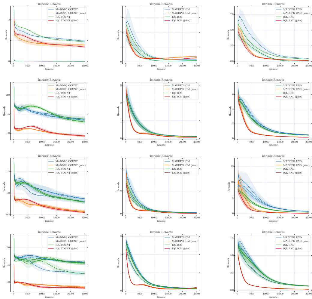
Figure C.21: Intrinsic rewards for MADDPG and IQL with individual and joint curiosities for cooperative communication (1st row), cooperative navigation (2nd row), physical deception (3rd row) and predator prey (4th row) task.
