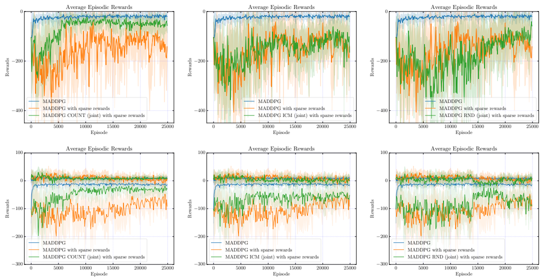
Figure 4.9: Episodic rewards for MADDPG with joint curiosities for cooperative communication (top) and physical deception (bottom) tasks with and without sparse rewards.
