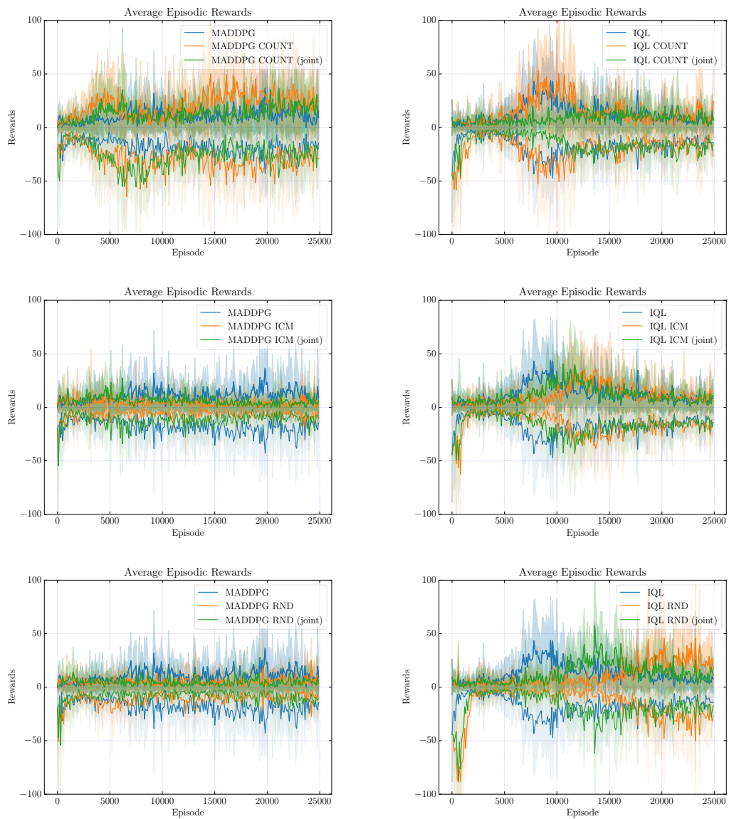
Figure C.4: Episodic rewards for MDDPG (left column) and IQL (right column) with individual and joint curiosities for predator prey task.
