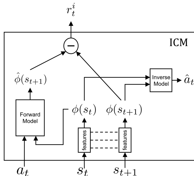
Figure 2.4: The ICM learns feature representation \phi for states through the inverse model predicting applied action a_t . A prediction \hat{\phi}(s_{t+1}) of the upcoming state representation is computed using the forward model. Figure taken from Pathak et al. [2017]
