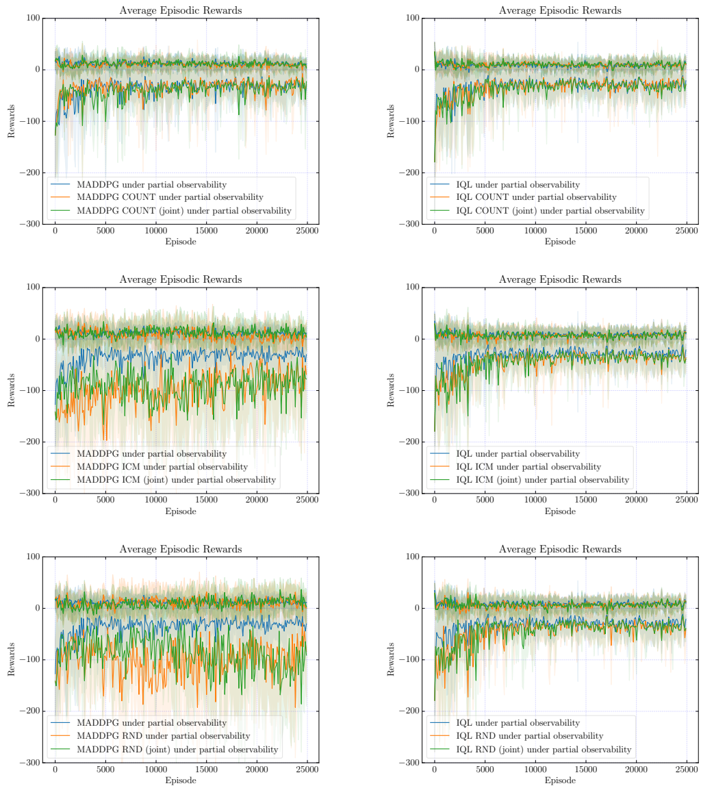
Figure C.9: Episodic rewards for MADDPG (left column) and IQL (right column) with individual and joint curiosities for physical deception task under partial observability.
