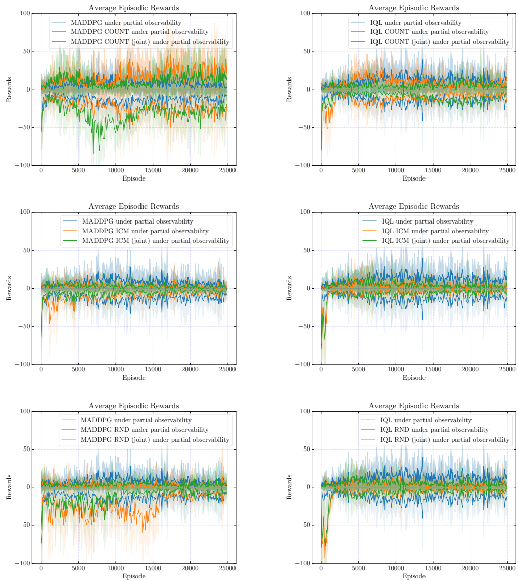
Figure C.11: Episodic rewards for MADDPG (left column) and IQL (right column) with individual and joint curiosities for predator prey task under partial observability.
