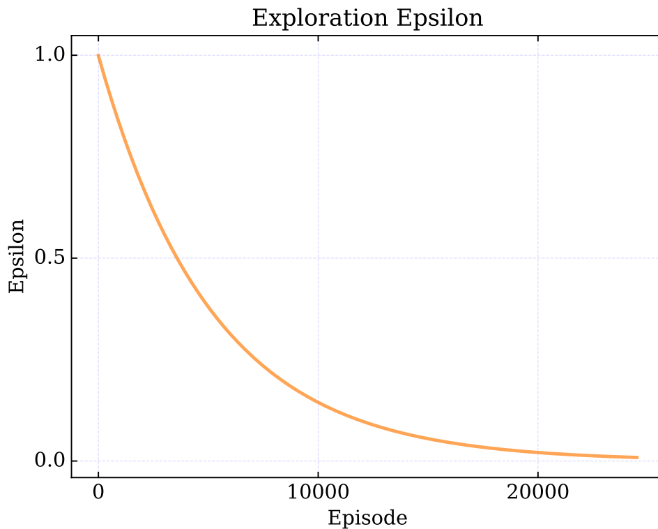
Figure B.1: \epsilon -decay for 25,000 episodes each having 25 steps.
