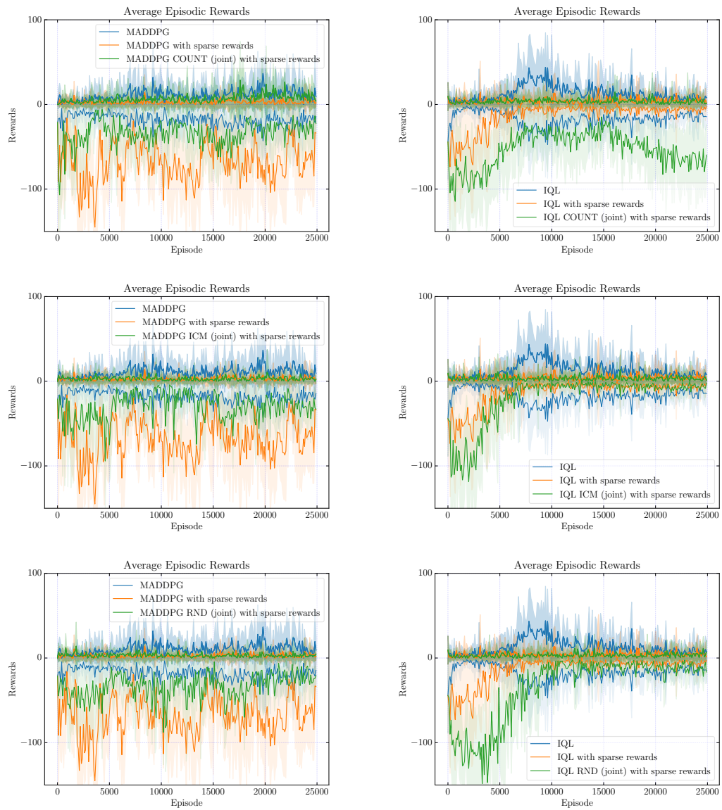
Figure C.20: Episodic rewards for MADDPG (left column) and IQL (right column) with joint curiosities for predator prey task with and without sparse rewards.
