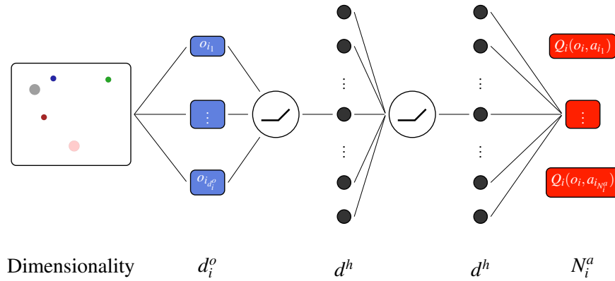
Figure 3.1: Illustration of DQN architecture for agent i with two intermediate layers of hidden representation size d^h and ReLU activation function.
