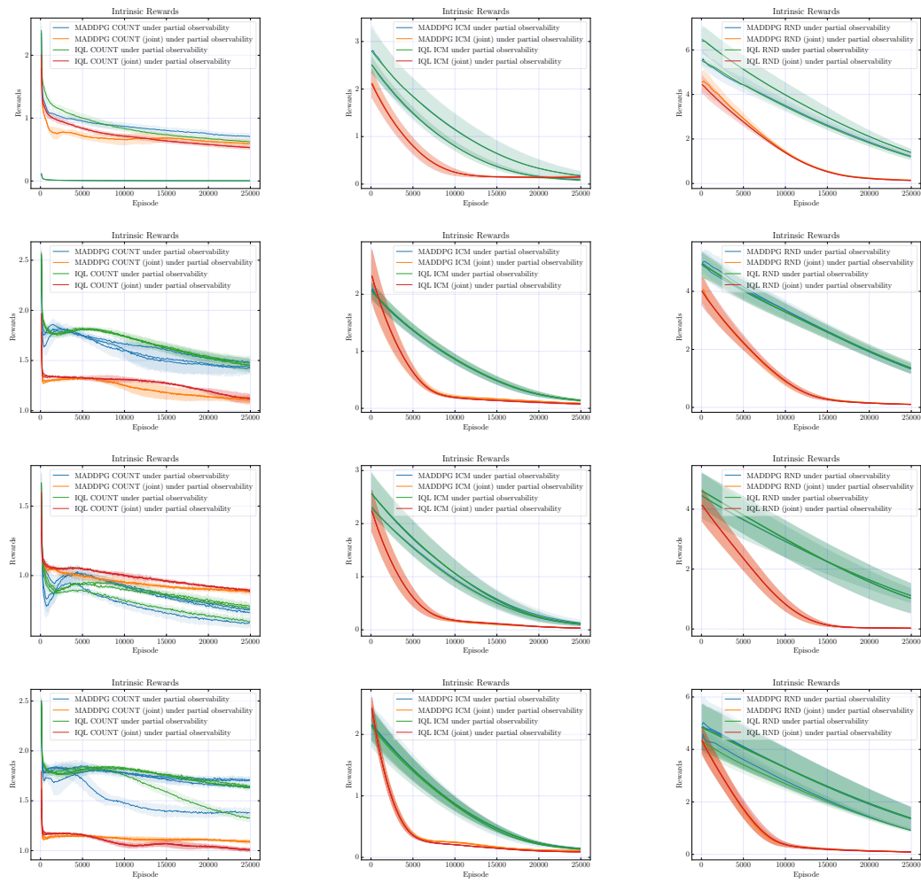
Figure C.22: Intrinsic rewards for MADDPG and IQL with individual and joint curiosities for cooperative communication (1st row), cooperative navigation (2nd row), physical deception (3rd row) and predator prey (4th row) task under partial observability.
