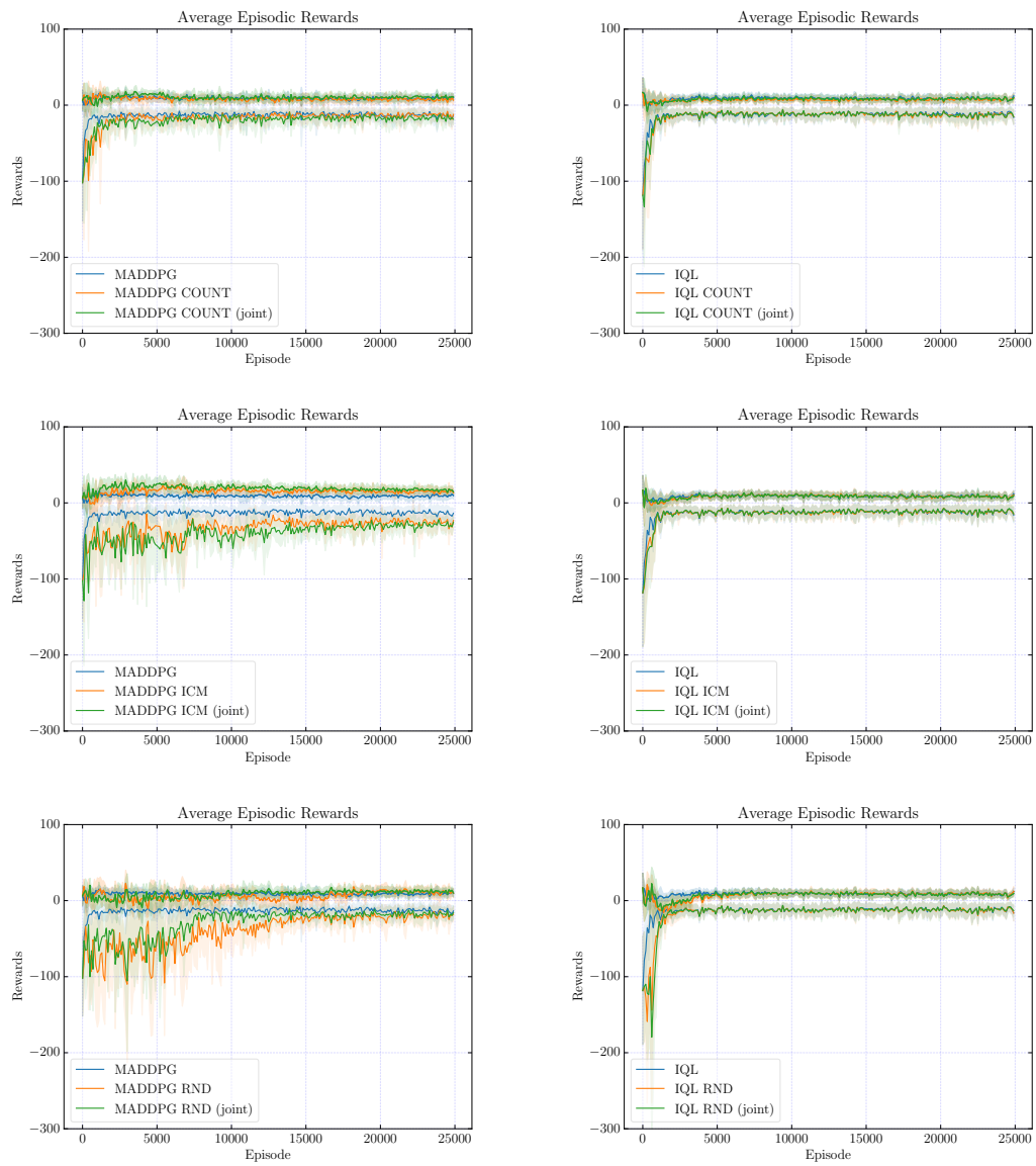
Figure C.3: Episodic rewards for MDDPG (left column) and IQL (right column) with individual and joint curiosities for physical deception task.
