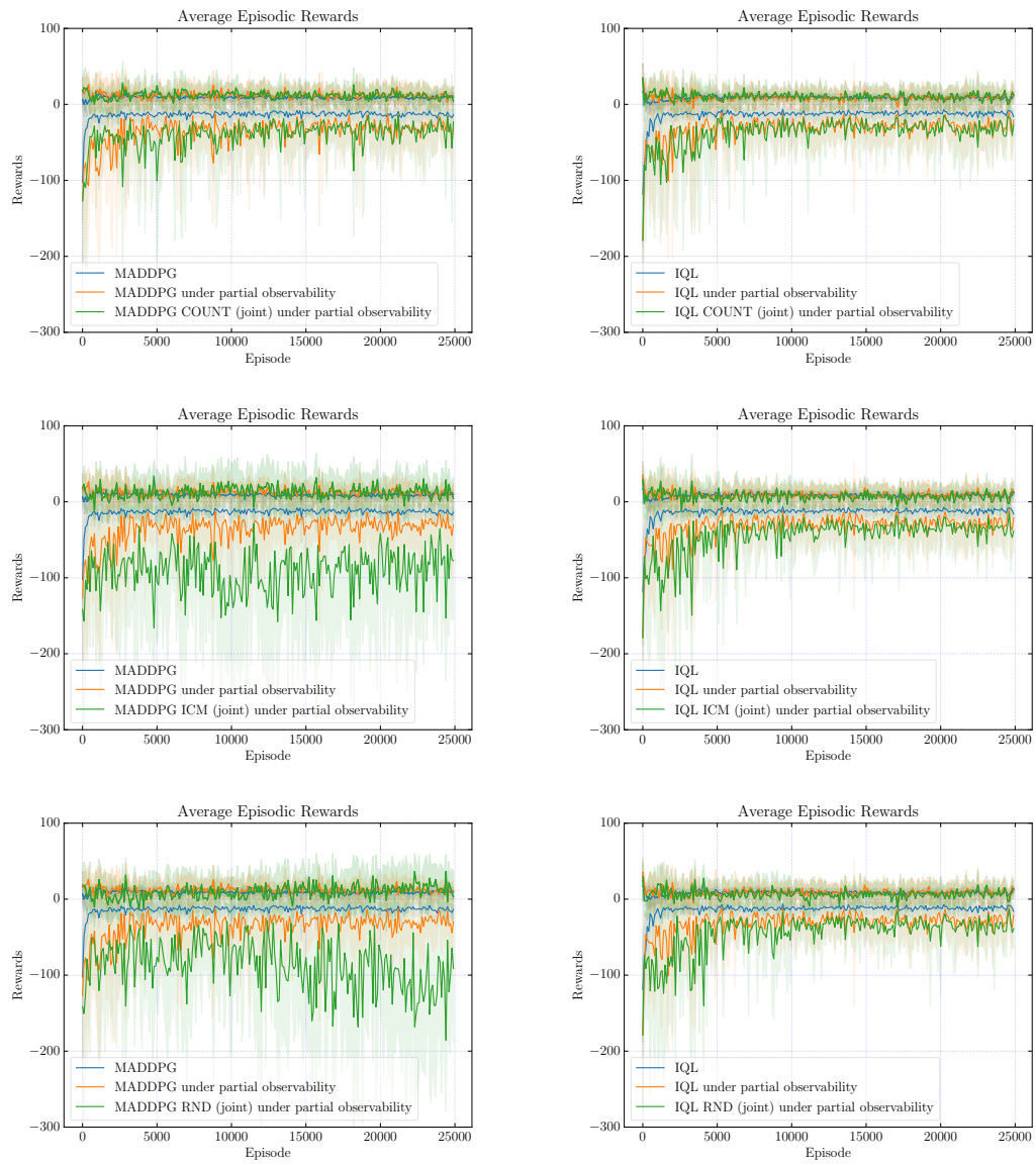
Figure C.10: Episodic rewards for MADDPG (left column) and IQL (right column) with joint curiosities for physical deception task with and without partial observability.
