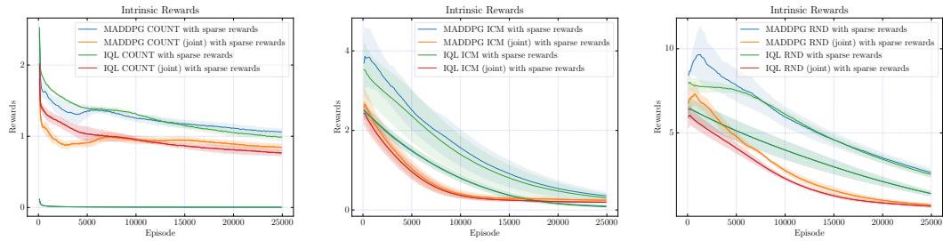
Figure 4.10: Intrinsic rewards for MADDPG and IQL with individual and joint curiosities for cooperative communication task with sparse rewards.
