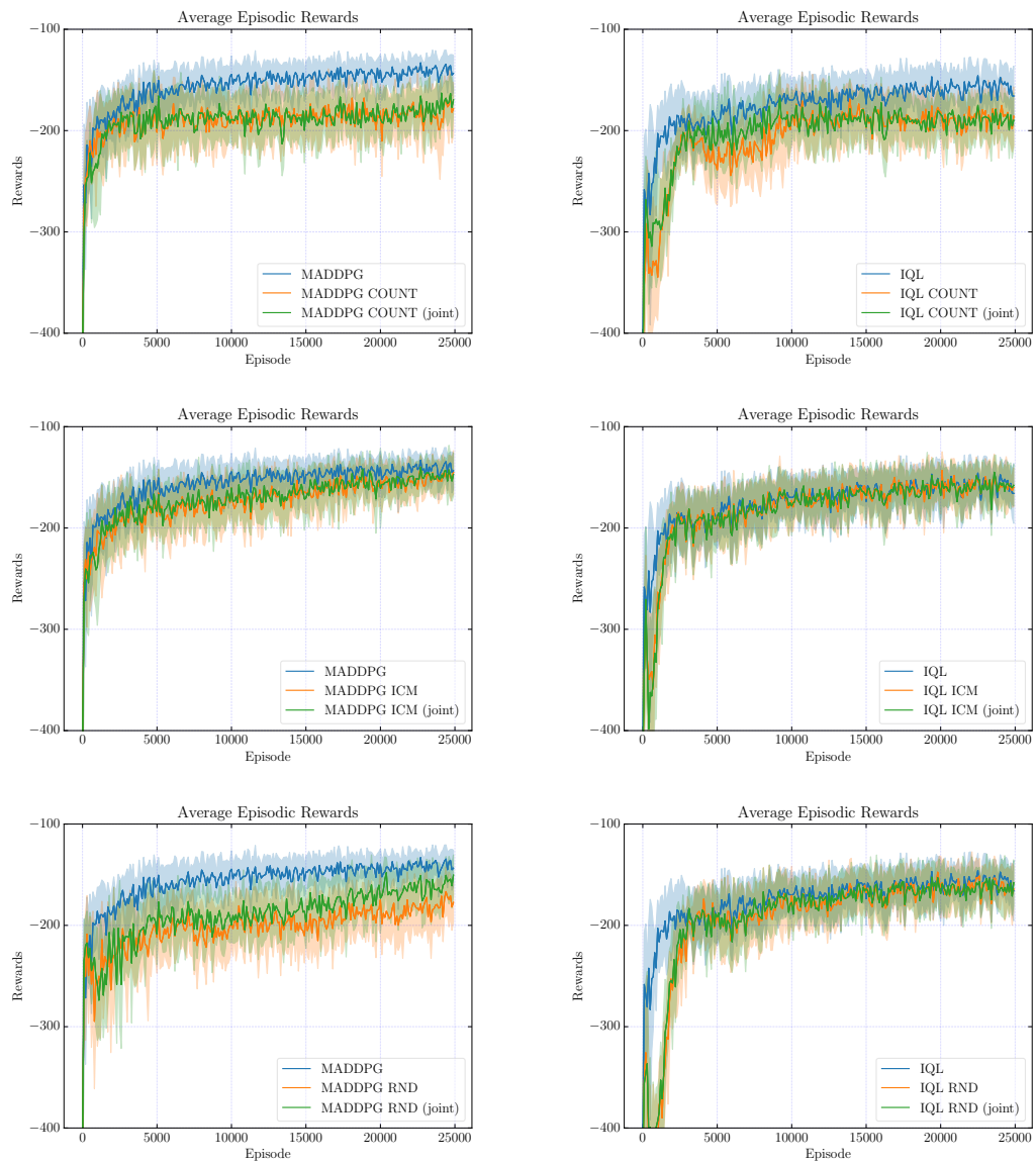
Figure C.2: Episodic rewards for MDDPG (left column) and IQL (right column) with individual and joint curiosities for cooperative navigation task.
