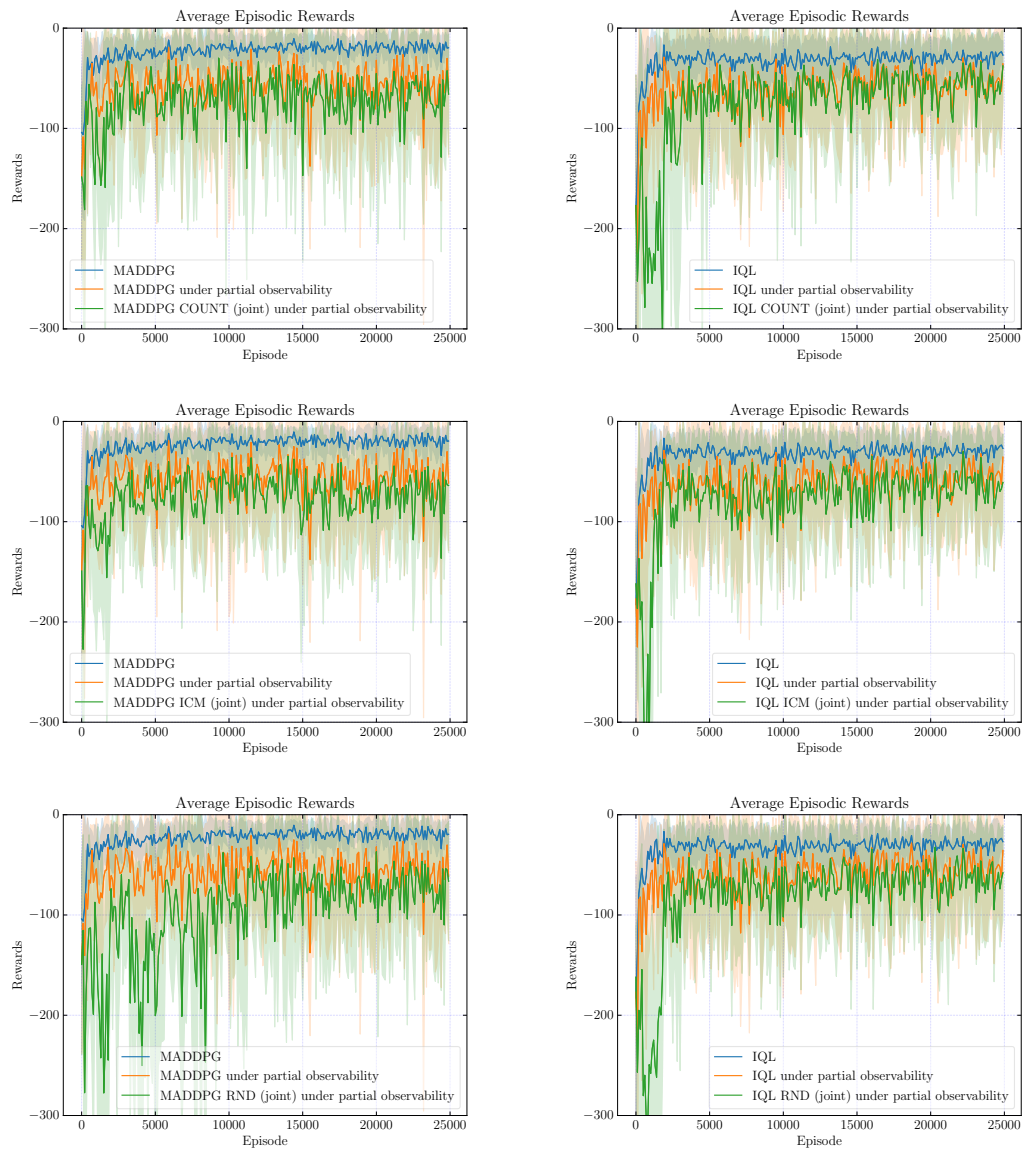
Figure C.6: Episodic rewards for MADDPG (left column) and IQL (right column) with joint curiosities for cooperative communication task with and without partial observability.
