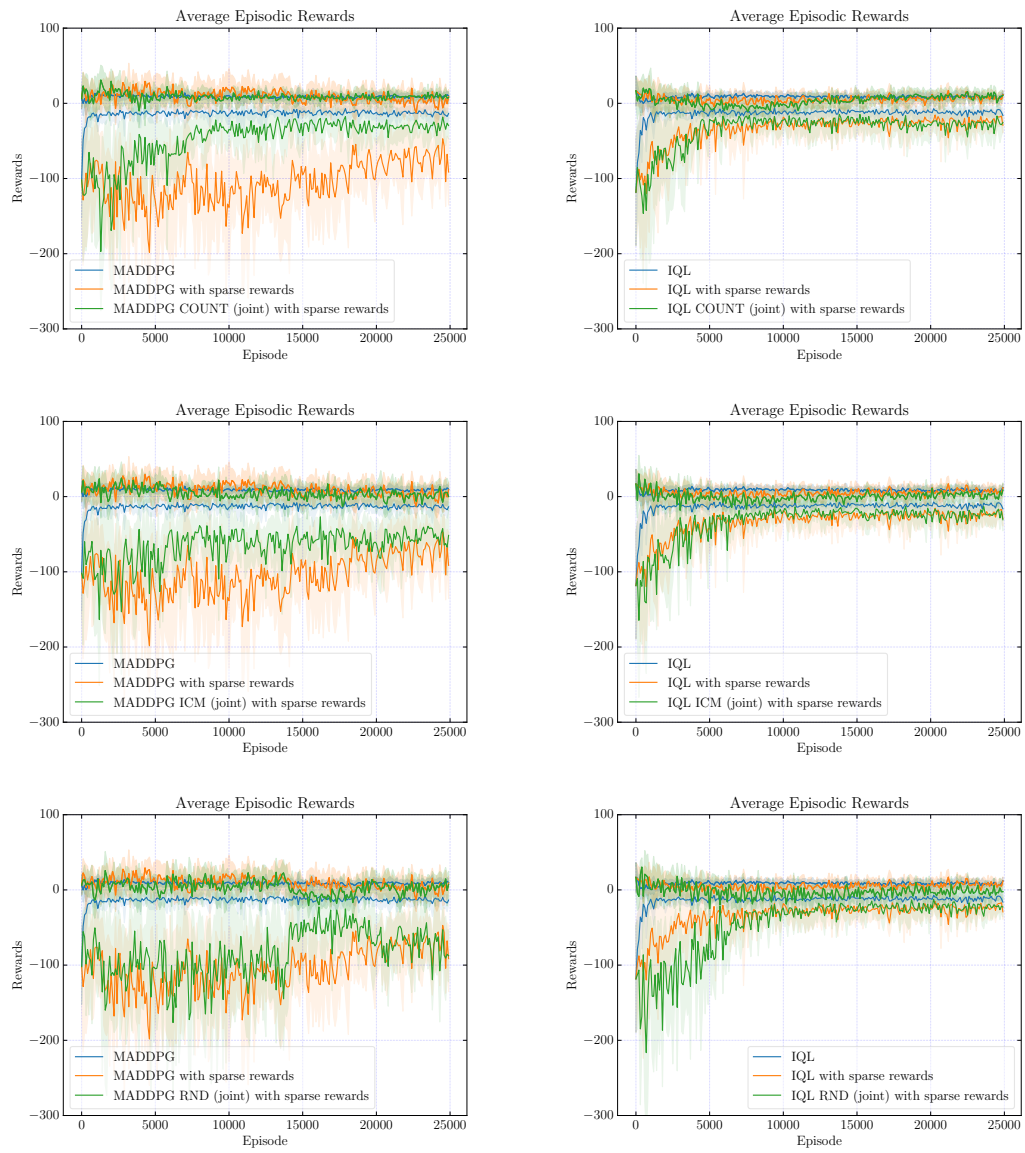
Figure C.18: Episodic rewards for MADDPG (left column) and IQL (right column) with joint curiosities for physical deception task with and without sparse rewards.
