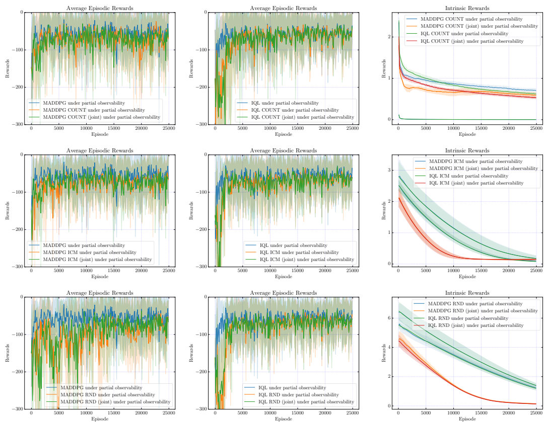
Figure 4.8: Episodic reward of MDDPG (left) and IQL (right) with individual and joint count (top), ICM (middle) and RND (bottom) curiosity on the cooperative communication task under partial observability. The right images show intrinsic rewards for MDDPG and IQL with the respective curiosity applied individually and jointly.
