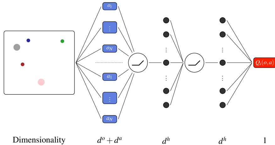
Figure 3.2: Illustration of MADDPG critic architecture for agent i with two intermediate layers of hidden representation size d^h and ReLU activation function. The action-value output is over the joint observations o = (o_1, \dots, o_N) and actions a = (a_1, \dots, a_N) .
