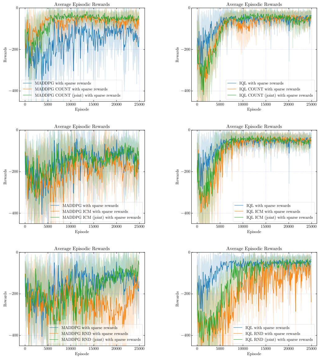
Figure C.13: Episodic rewards for MADDPG (left column) and IQL (right column) with individual and joint curiosities for cooperative communication task with sparse rewards.
