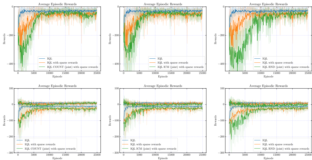
Figure 4.11: Episodic rewards for IQL with joint curiosities for cooperative communication (top) and physical deception (bottom) tasks with and without sparse rewards.
