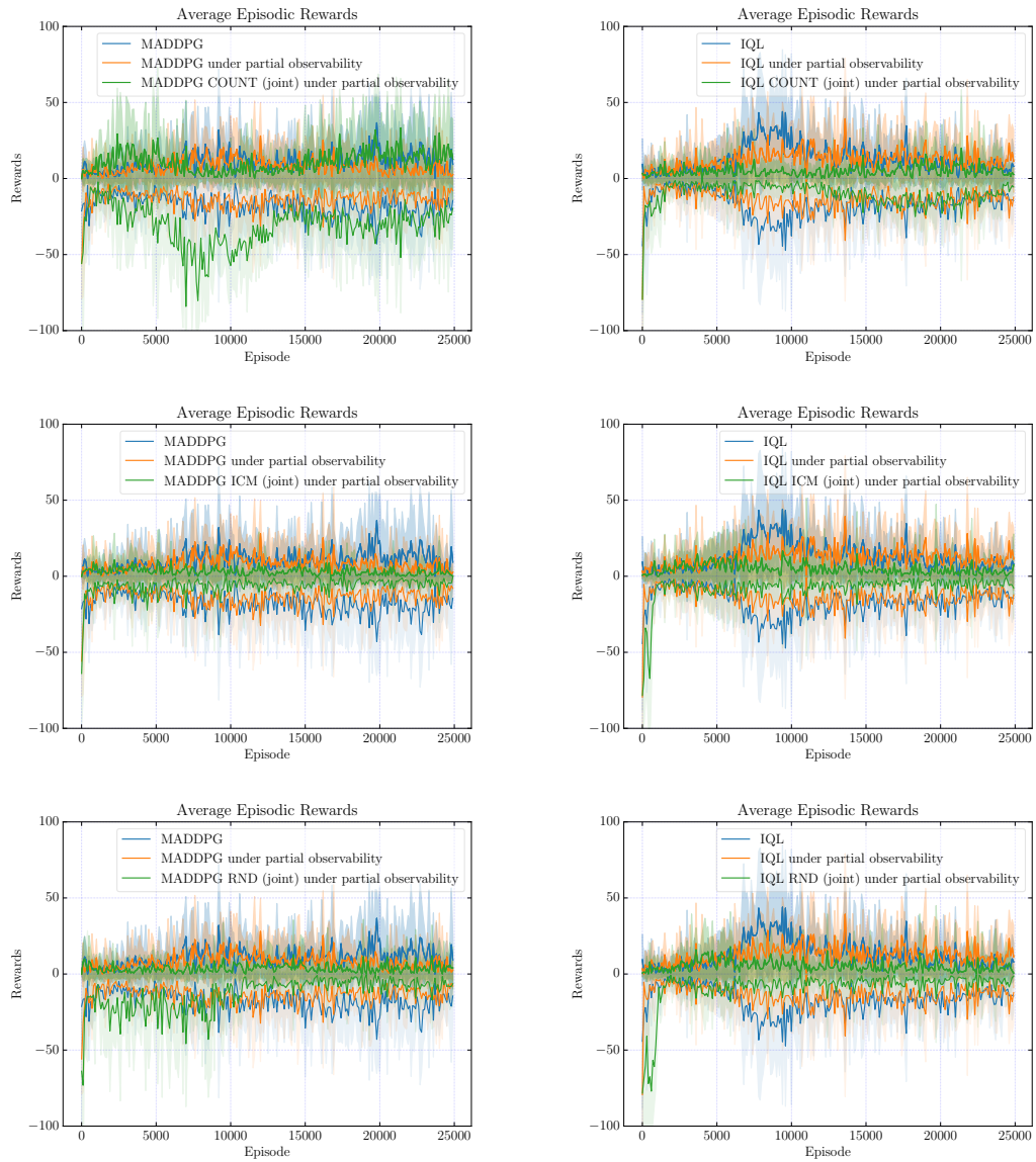
Figure C.12: Episodic rewards for MADDPG (left column) and IQL (right column) with joint curiosities for predator prey task with and without partial observability.
