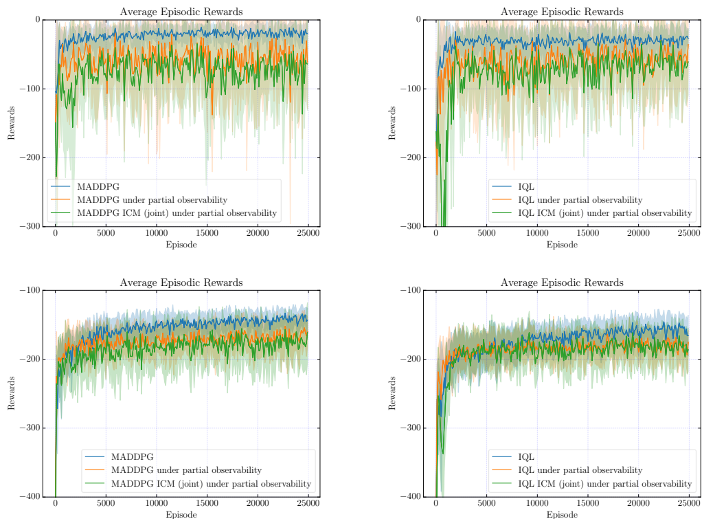
Figure 4.7: Episodic rewards for MADDPG (left) and IQL (right) with joint ICM curiosity for cooperative communication (top) and cooperative navigation (bottom) task with and without partial observability.
