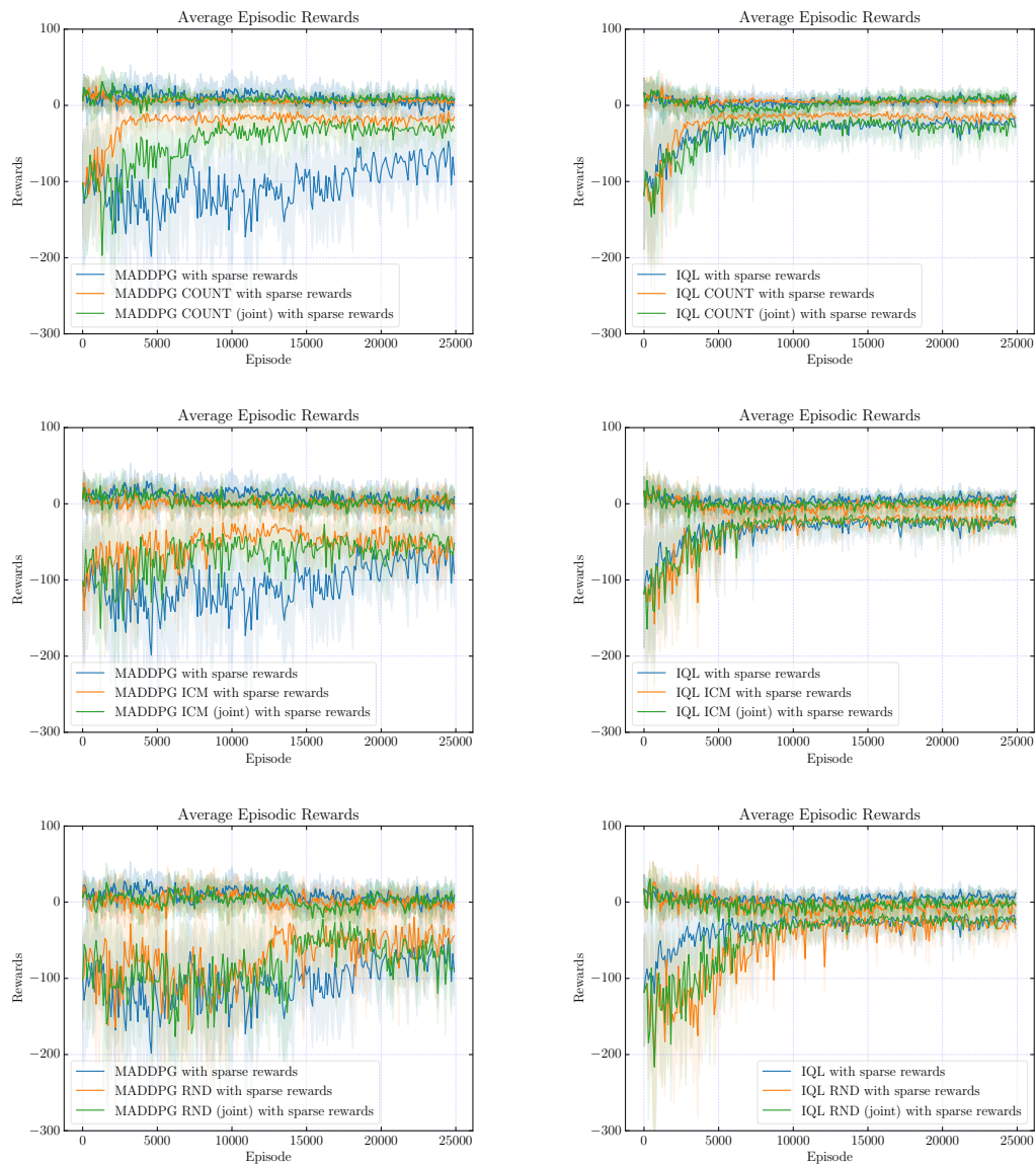
Figure C.17: Episodic rewards for MADDPG (left column) and IQL (right column) with individual and joint curiosities for physical deception task with sparse rewards.
